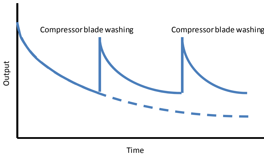
Figure 11.2-2 Efficiency recovery by offline compressor wash
