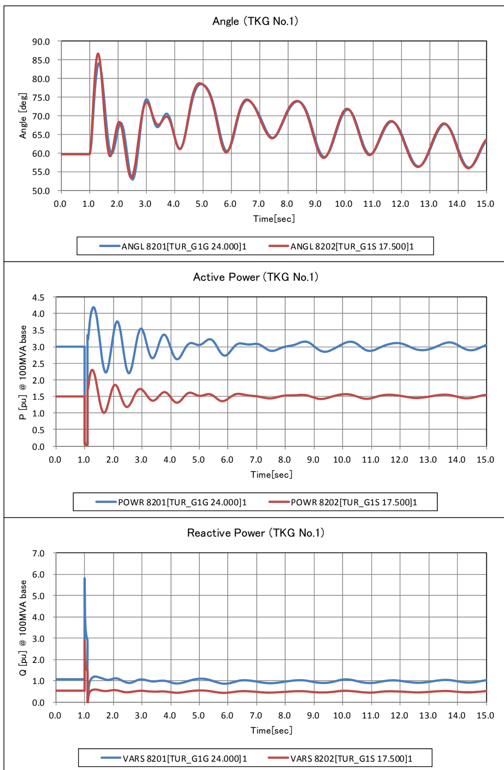
Fig. 7.1.5-1 Result of Case 1 (1/3)
