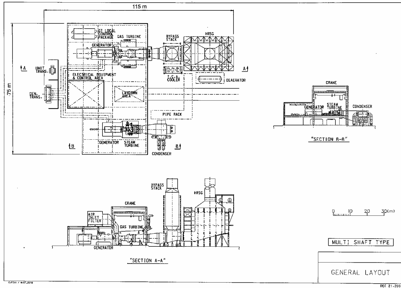
Figure 6.1.3-3 Typical Layout of One (1) Unit of Multi-shaft Configuration CCPP
