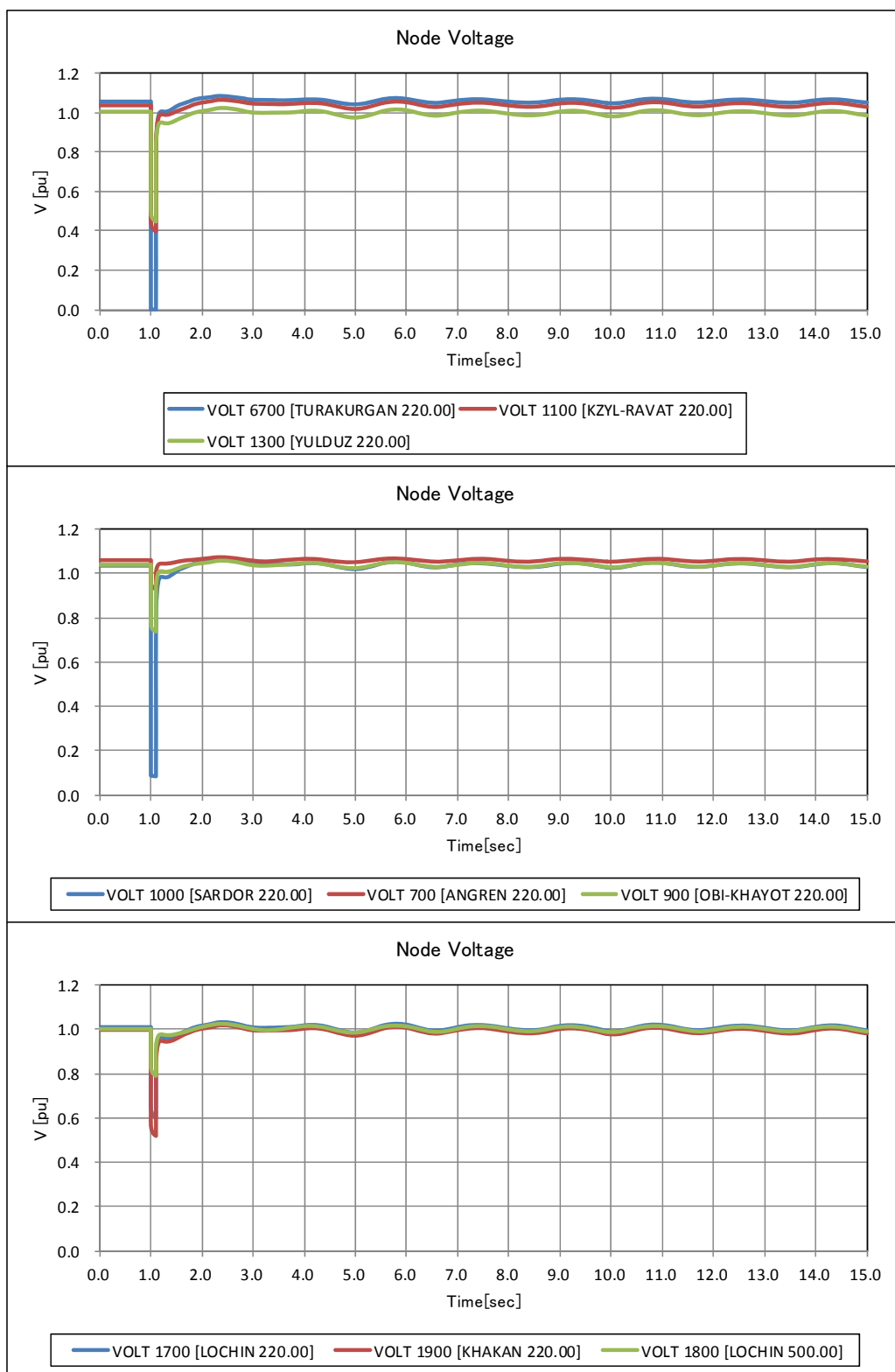
Fig. 7.1.5-3 Result of Case 1 (3/3)
