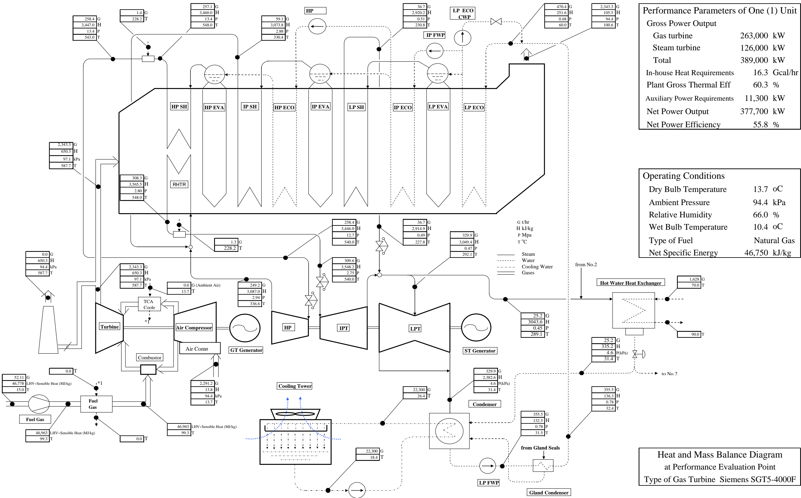
Figure 6.1.5-4 Heat and Mass Balance Diagram of One (1) Unit of CCPP by Siemens SGT5-4000F Gas Turbine
