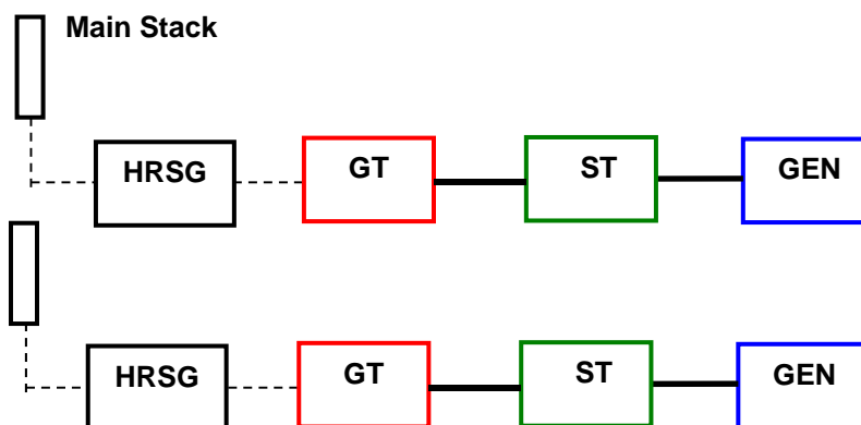
Figure 6.1.3-1 Shaft Configuration
