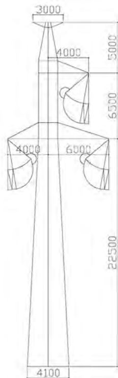
Source: JICA Study Team Figure 7.2.3-2 Type “SS” Tower
