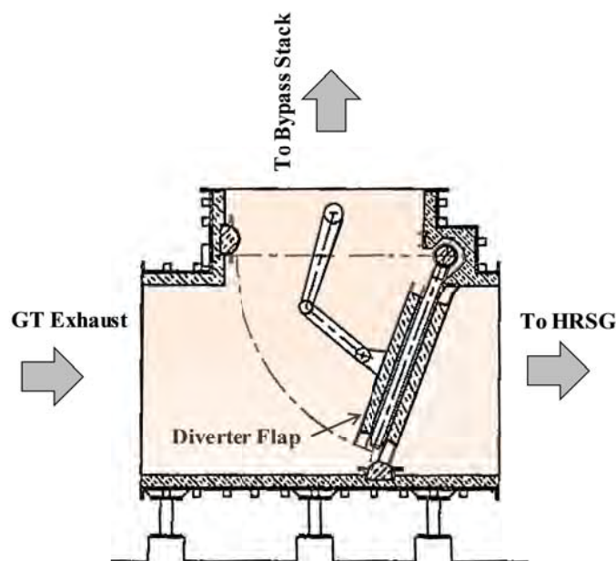
Figure 6.3.3-2 Diverter Damper
