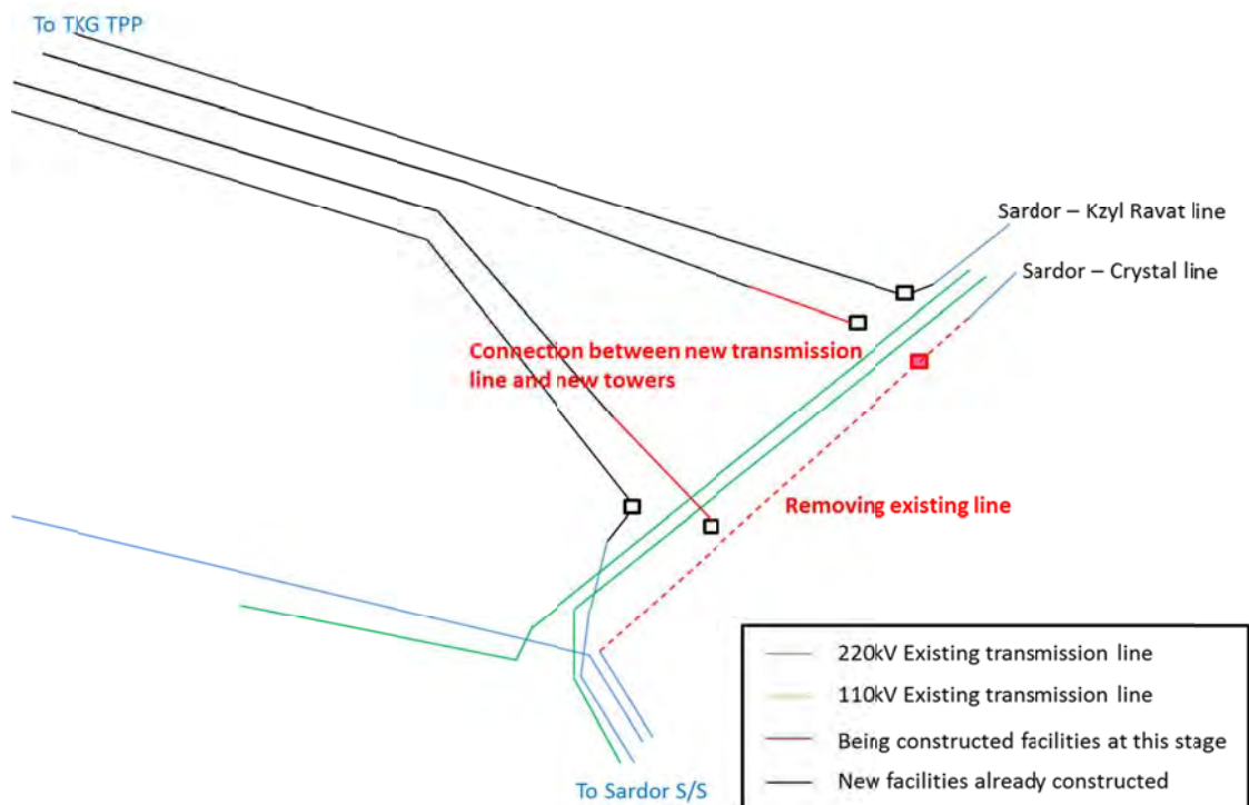
Figure 7.2.4-6 The 4-cct T/L Connection Procedure to the Existing Power Grid (6)
