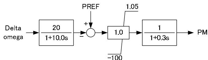
Fig. 7.1.2-5 Block Diagram of Governor (IESGO for HPP)
