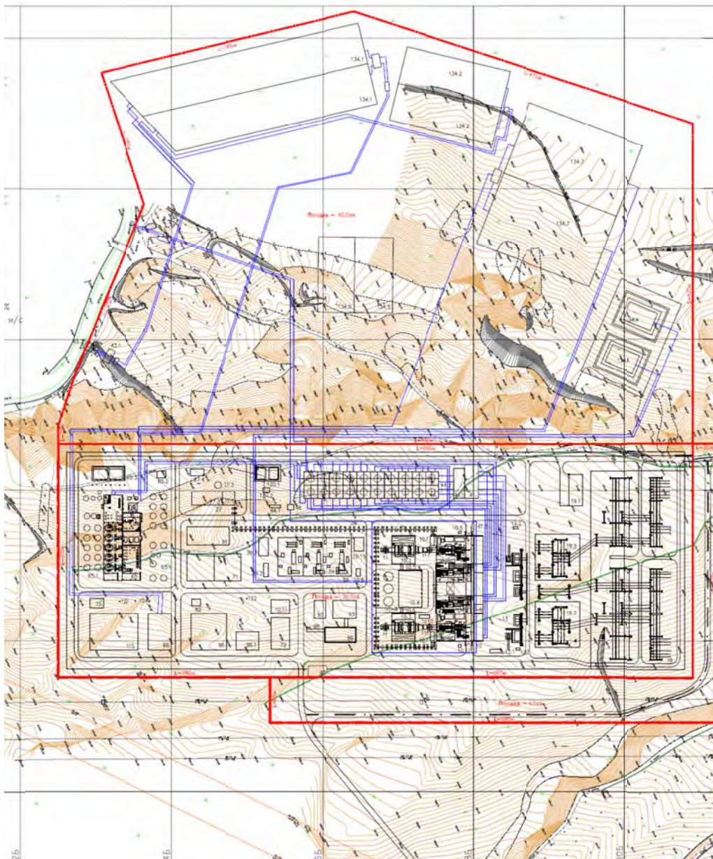
Figure 6.3-1 Plot plan
