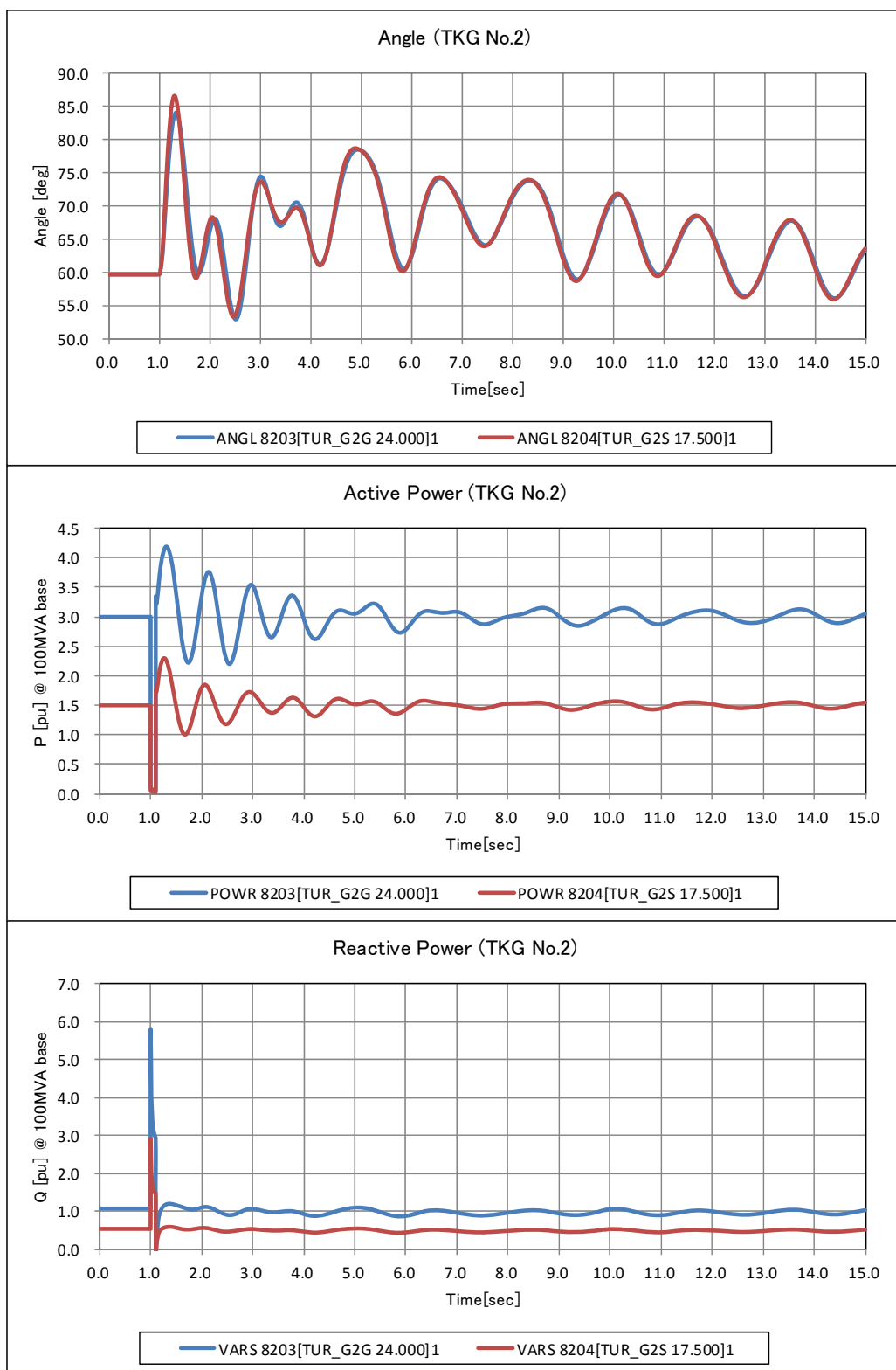
Fig. 7.1.5-2 Result of Case 1 (2/3)
