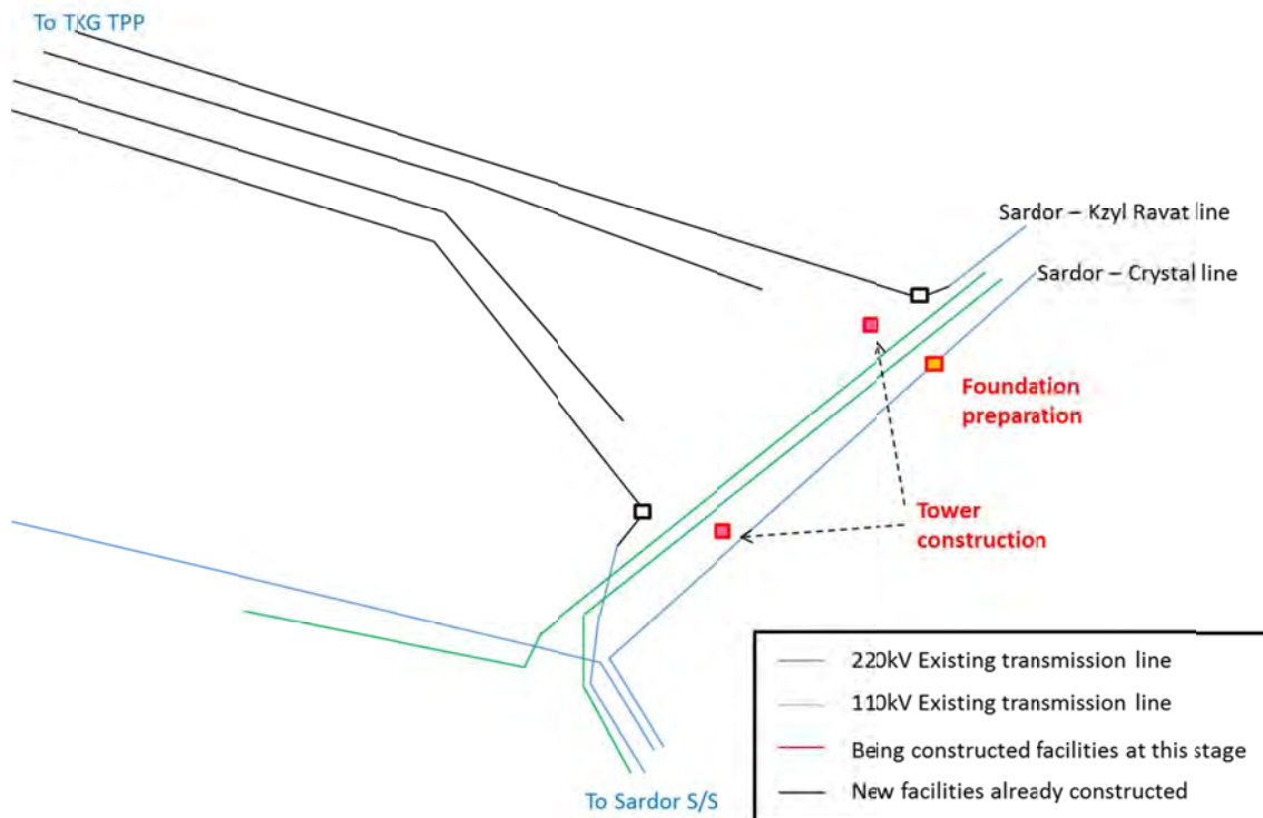
Figure 7.2.4-5 The 4-cct T/L Connection Procedure to the Existing Power Grid (5)
