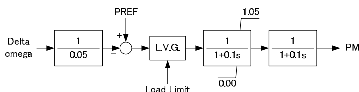
Fig. 7.1.2-6 Block Diagram (GAST for GT)
