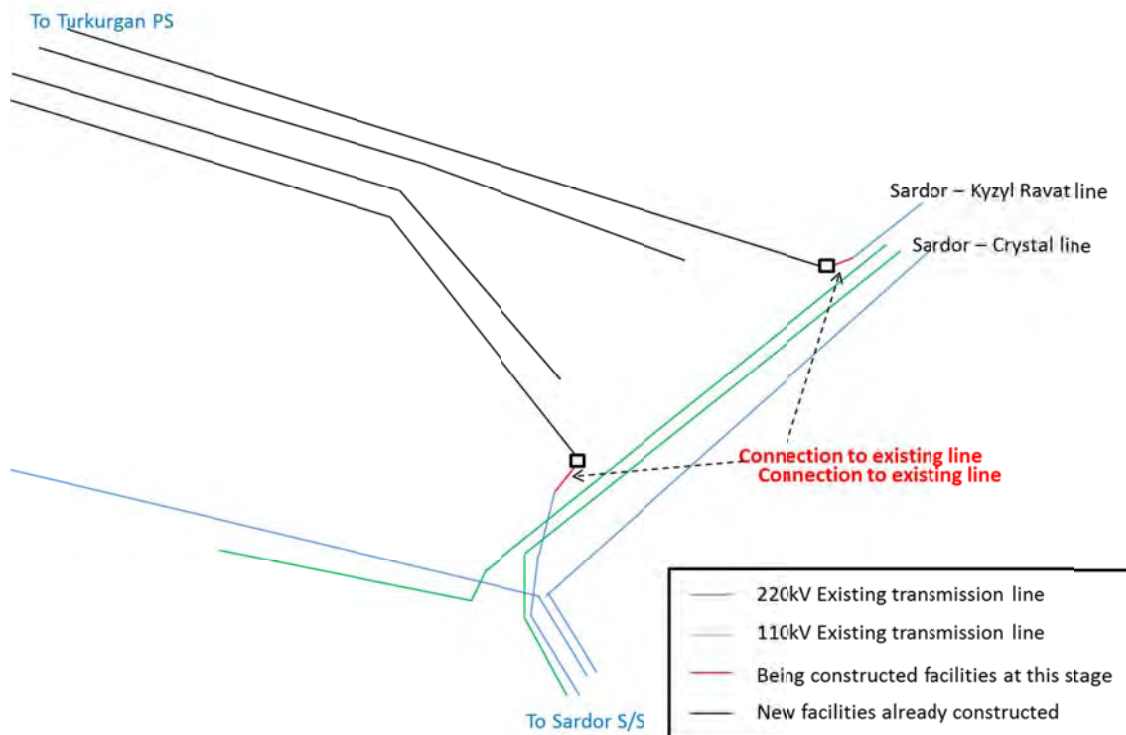
Figure 7.2.4-4 The 4-cct T/L Connection Procedure to the Existing Power Grid (4)
